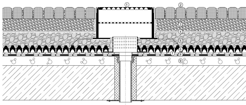
(1)TGS inspection box, (2)paved area, (3)Bedding, (4)VLF filter geotextile, (5)supporting layer, (6)DiaDrain-60 drainage board,(7)VLU mechanical protection layer,(8)Root resistant waterproofing membrane, (9) Roof construction
