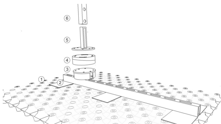
(1)MDE-60 Mounting Board, (2)Base Rail, (3)Base Plate, (4)Tilting Screw, (5)Hosting Element, (6)Fence post
