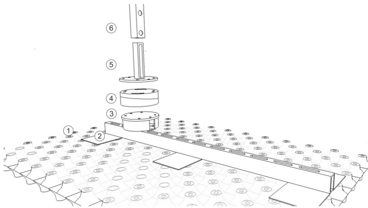
(1)MDE-60 Mounting Board, (2)Base Rail, (3)Base Plate, (4)Tilting Screw, (5)Hosting Element, (6)Fence post
