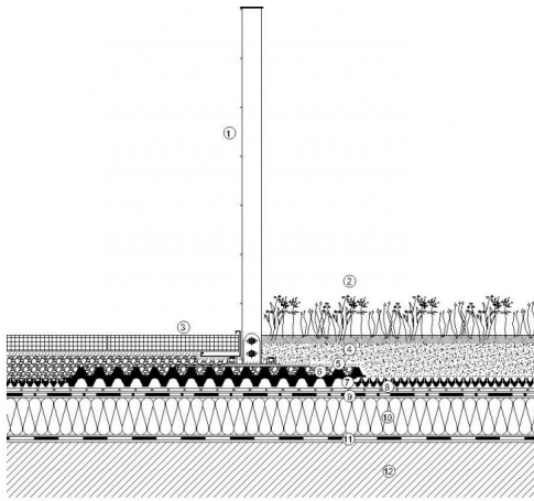
(1)ADZ Fencing System, (2)Vegetation, (3)Paving slab, (4)Substrate, (5)VLF filter geotextile, (6)Gravel, (7)MDE-60 mounting board, (8)VLU mechanical protection geotextile, (9)Waterproofing membrane, (10)Thermal insulation layer, (11)Vapour control layer, (12)Roof construction
