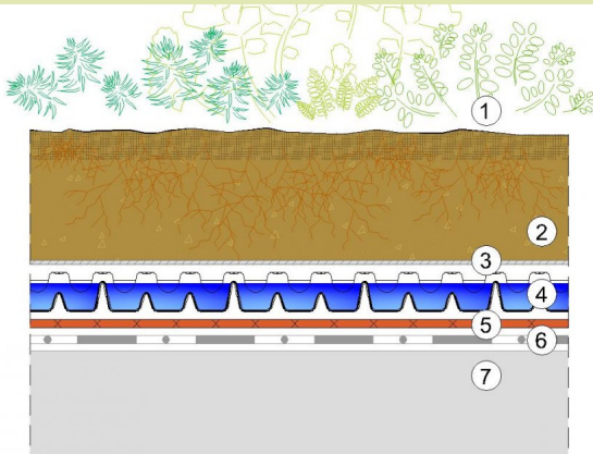
(1)Vegetation, (2)Growing media, (3)VLF 150/200 filter layer, (4)DiaDrain-40H, (5)VLU 300/500 mechanical protection layer, (6)Root resistant waterproofing membrane, (7)Roof construction
