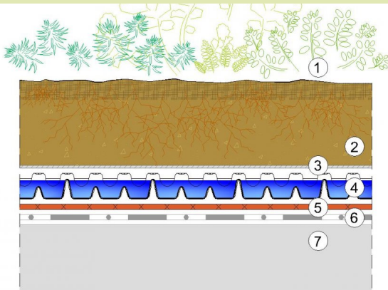
(1)Vegetation, (2)Growing media:6", (3)VLF 150/200 filter layer:1/16", (4)DiaDrain-25H:1", (5)VLU 300/500 mechanical protection layer:1/16", (6)Root resistant waterproofing membrane:-, (7)Roof construction
